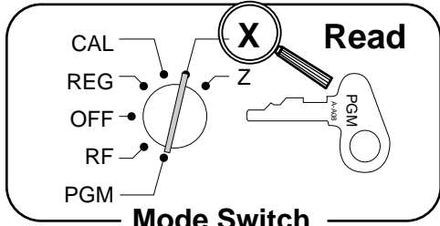
Mode Switch
